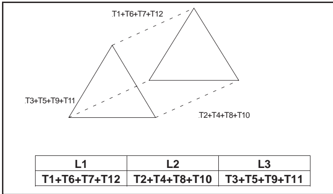
12 Lead 230V Connection
